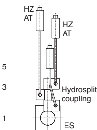
Mounting style 1
